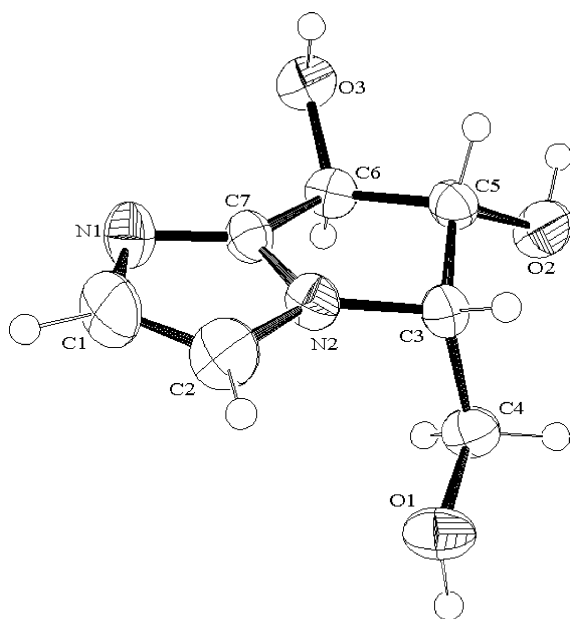
Figure 3. ORTEP plot of the structure of ent - 8 (50% probability ellipsoids).
