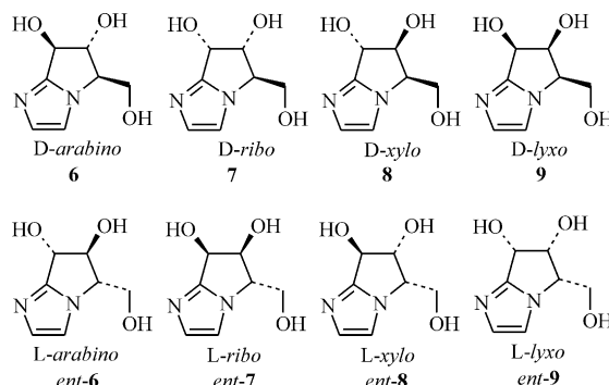
Figure 2. The eight imidazolo-[1,2]-pyrrolidinoses.
