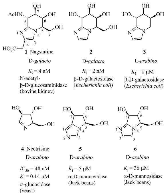
Figure 1. Various imidazolosugar inhibitors of glycosidases.
