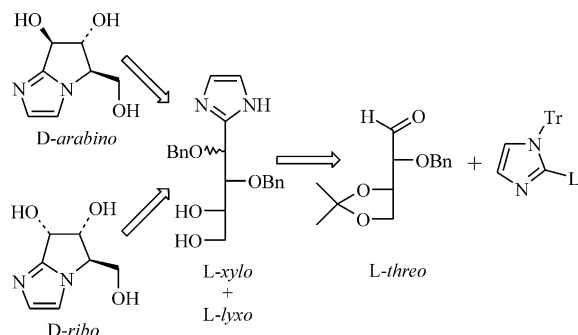
Scheme 1. Retrosynthetic pathway for both the D -arabino- and D -ribo-imidazolo-[1,2]-pyrrolidinoses.
